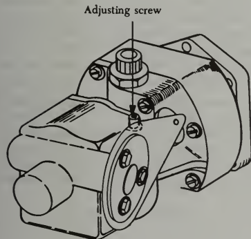
FIGURE 7-24. Propeller r.p.m. adjusting screw.
